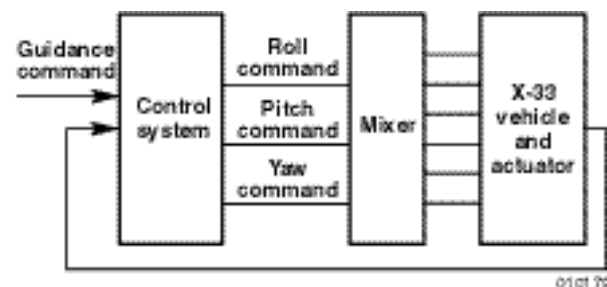
Figure 3. X-33 entry flight control.
